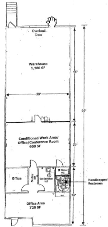
Floor Plan
